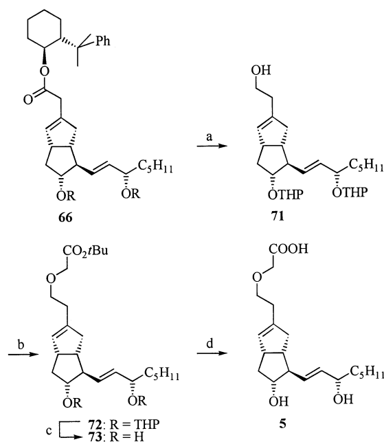
Scheme 15
