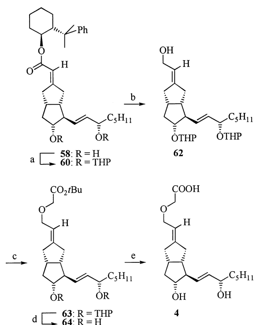
Scheme 13
