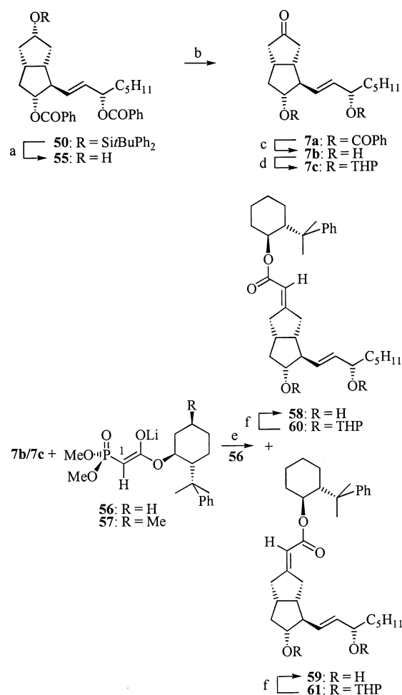
Scheme 12
